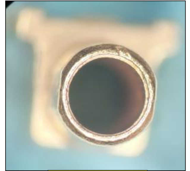
"OK" Part
